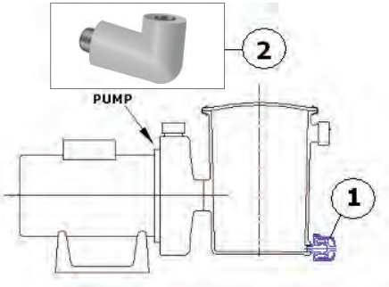
Figure 1. Breather II-ADJ System Schematic
